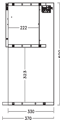
Haut mini-four
