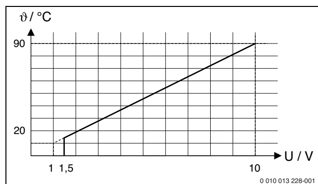
Fig. 2 Linear relationship between the 0-10 V signal ( U in volts) and the demanded flow temperature \theta (in °C with reference to the minimum flow temperature range to the maximum flow temperature range [default setting 20 °C to 90 °C])
