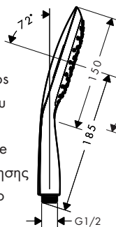
Raindance Select E 150 3jet 26551000 / 26551400
