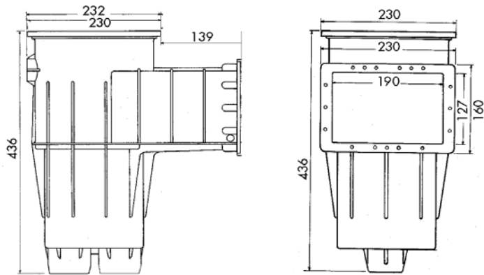
SKIMMER BETON PM SK11BP
