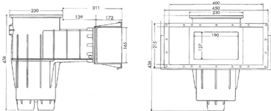
SKIMMER LINER GM SK11L
