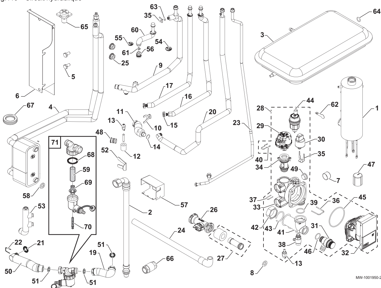
Fig.110 Circuit hydraulique
