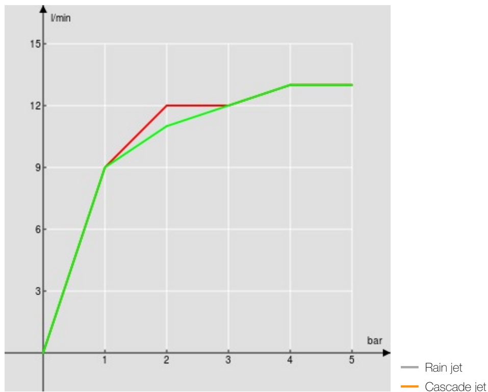
FLOW RATE DIAGRAM: HOT/COLD WATER
