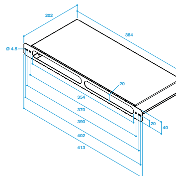
Encombrement MEA 85
