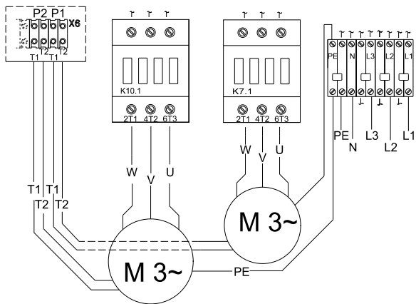
Fig. 9 Multilift MD/MLD.22.3.4
