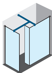
KUADRA H x2 KUADRA HL STANDARD SUPPORT BAR (included)
