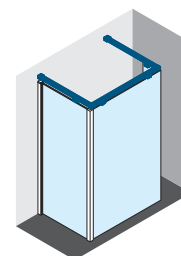
KUADRA HL x2 KUADRA H EVO FIXING SYSTEM (C-version)
