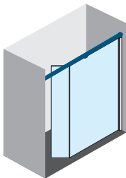
KUADRA H KUADRA HFA EVO FIXING SYSTEM (in recess)
