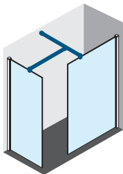
KUADRA H x2 STANDARD SUPPORT BAR (included)
