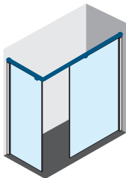
KUADRA H x2 EVO FIXING SYSTEM (corner version)
