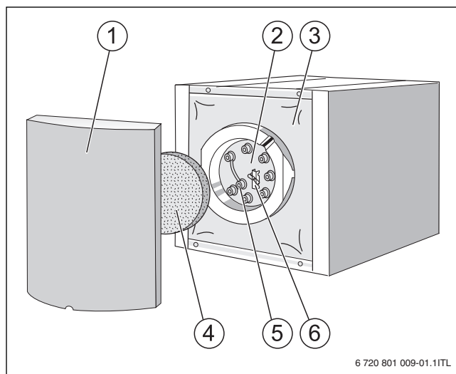
Sl.1 WST 135-2 HRC, WST 160-2 HRC i WST 200-2 HRC
