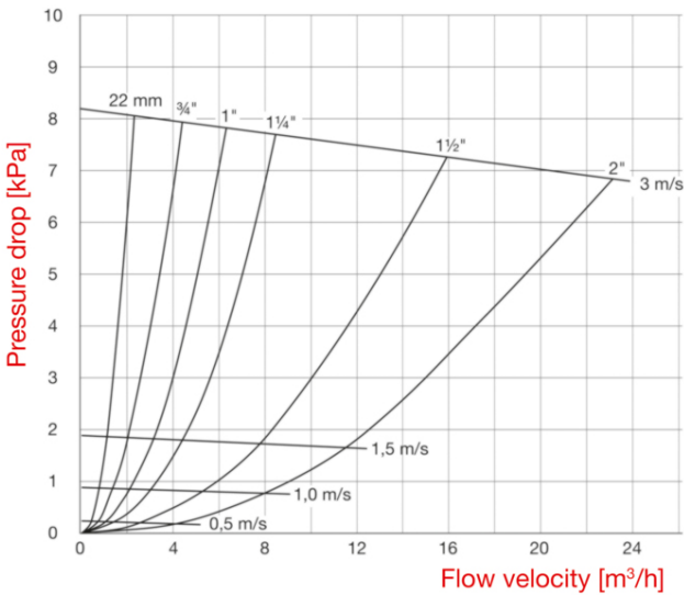
Selection table for Flamcovent & Clean Smart series
